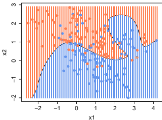
Lasso: min lambda decision boundary
