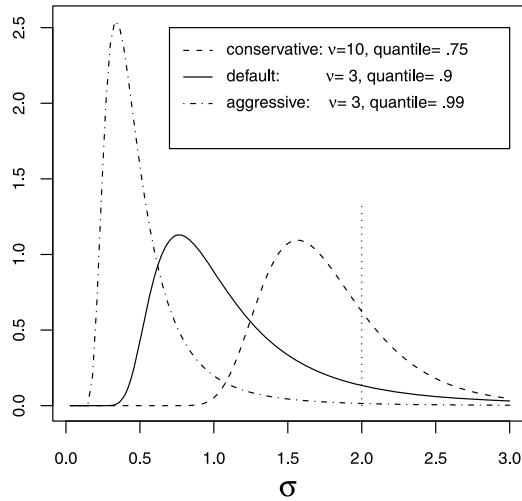
FIG. 1. Three priors on \sigma based on \text{df} = v and \text{quantile} = q when \hat{\sigma} = 2 .
